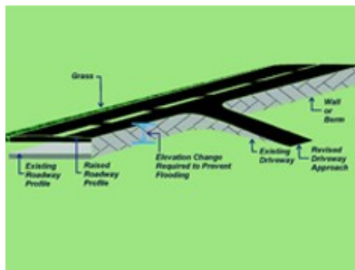
Raise Roadway Profile
